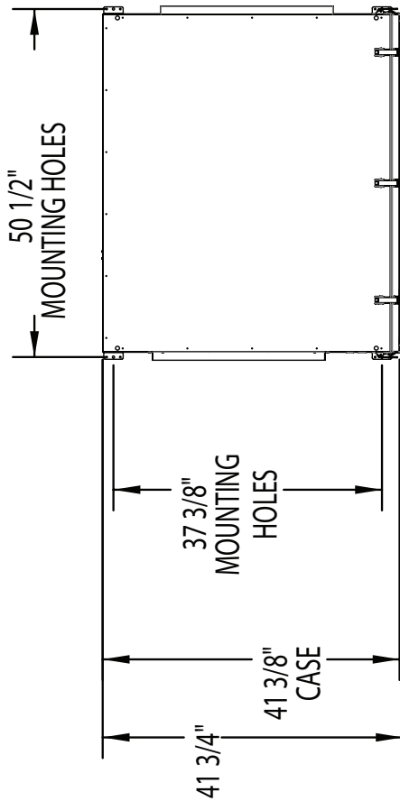
TOP VIEW
