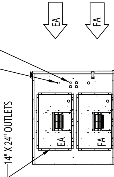
LEFT VIEW
