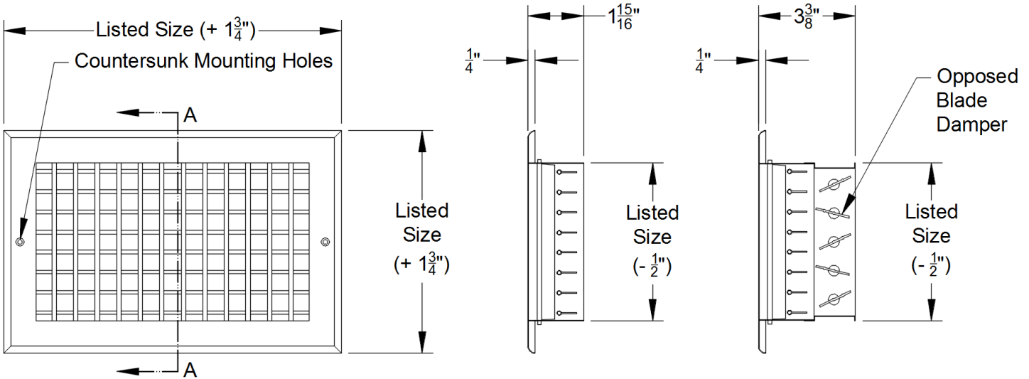
220V shown; all dimensions are typical for the 220 series
