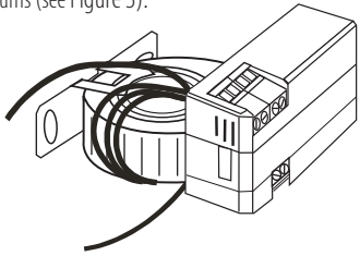
Figure 3: CSS Shown with Four Turns
