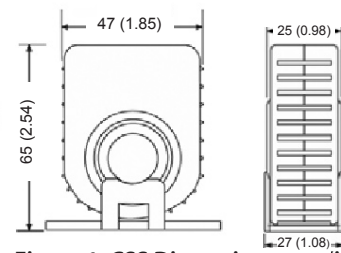
Figure 1: CSS Dimensions mm (in.)
