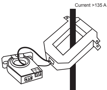
Figure 5: CSS with CT Transformer
