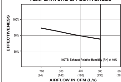
TEMPERATURE EFFECTIVENESS
