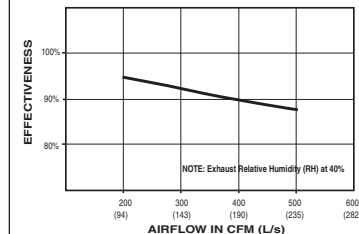
TEMPERATURE EFFECTIVENESS
