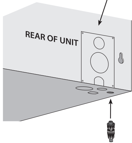
Bottle probe connector routing location
