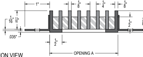
SECTION VIEW SCALE 1:2
