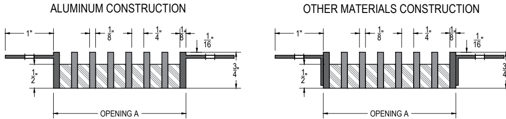
SECTION VIEW SCALE 1:2
